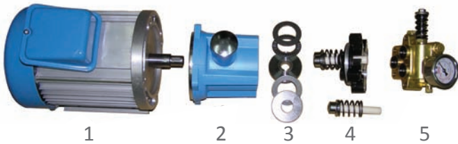
1/2HP, 1/3HP Pump break down
