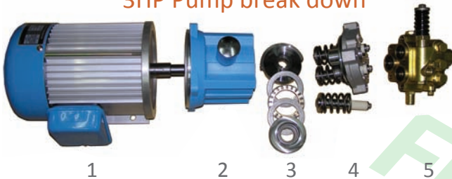
3HP Pump break down
