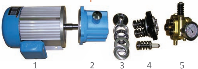
1HP Pump break down
